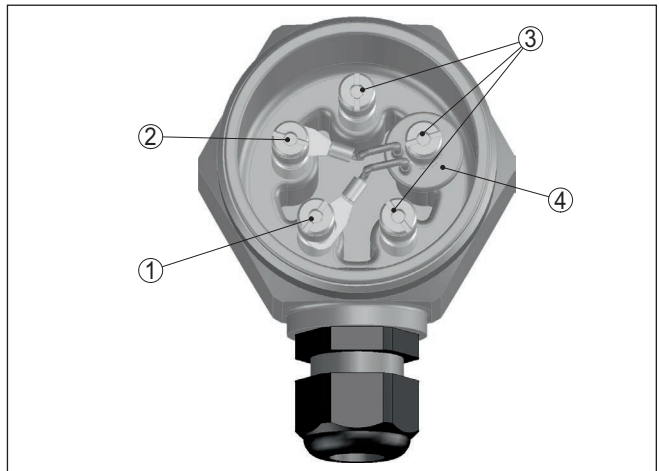
Fig. 6: Mounting of the additional electronics for line break monitoring
